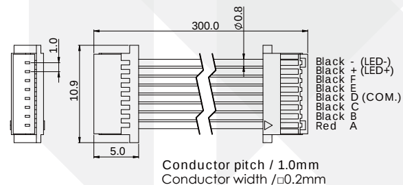
Cable: YCW014
